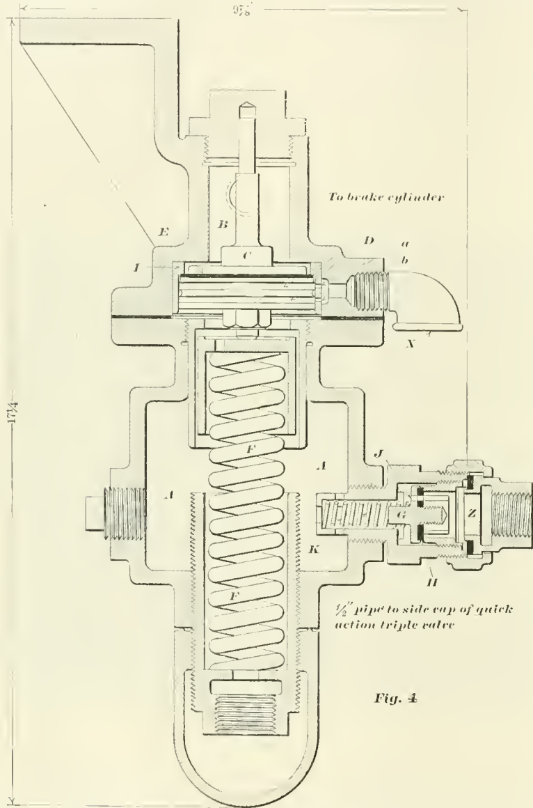
SECTIONAL VIEW OF NEW YORK AIR BRAKE COMPANY'S COMPENSATING VALVE FOR HIGH SPEED BRAKES.
